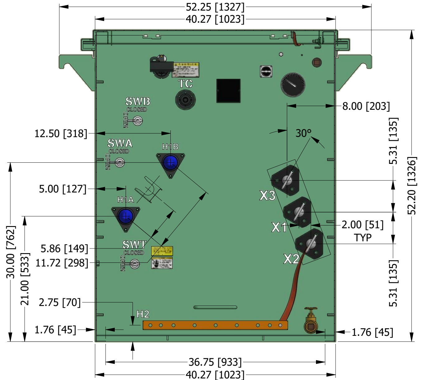
FRONT VIEW - SECTION A-A
