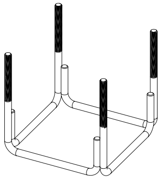
Fig. 1: Prefabricated anchor
